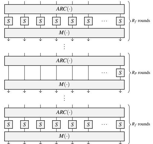
Figure 2: Construction of the HADES-based POSEIDON ^\pi permutation.
